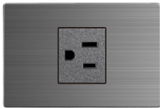
N5.2-011 1 Gang American socket 15A 125V 16A 250V
