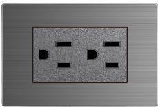
N5.2-012 2 Gang American socket 15A 125V 16A 250V
